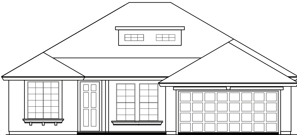
“A-4” ELEVATION-PLAN 1962
